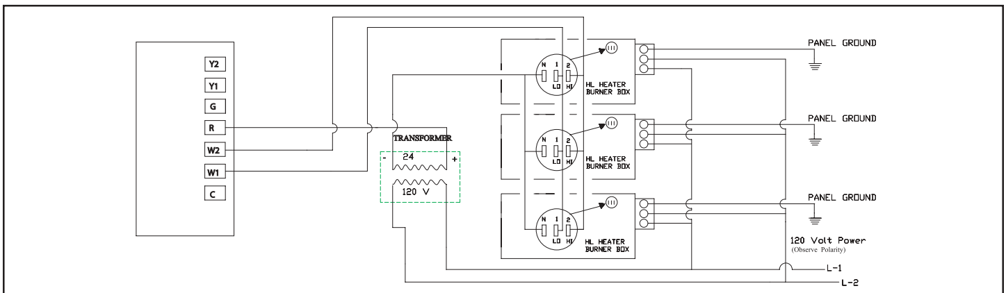
Two-stage heaters with a TH-1F81(261) thermostat. Multiple heaters, single thermostat. HLRB (relay boards) are installed.
