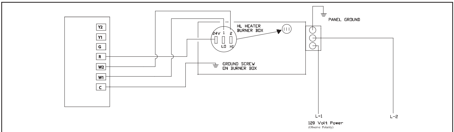
Two-stage heaters with a TH-1F81(261) thermostat. Single heater, single thermostat. No HLRB (relay board) is installed.
