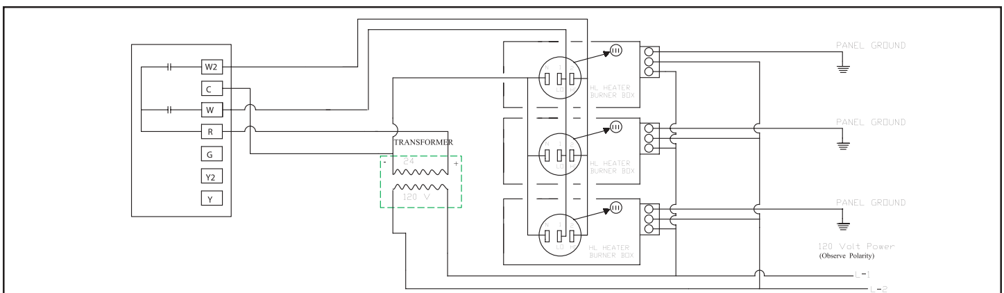
Two-stage heaters with a 1F81-51 thermostat. Multiple heaters, single thermostat. HLRB (relay boards) are installed.
