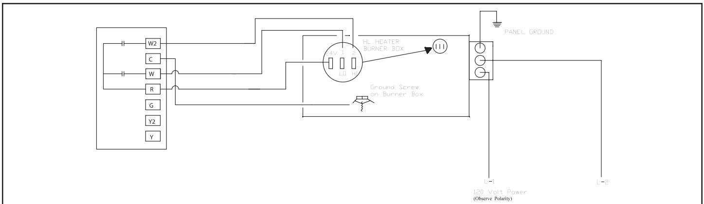
Two-stage heaters with a 1F81-51 thermostat. Single heater, single thermostat. No HLRB (relay board) is installed.
