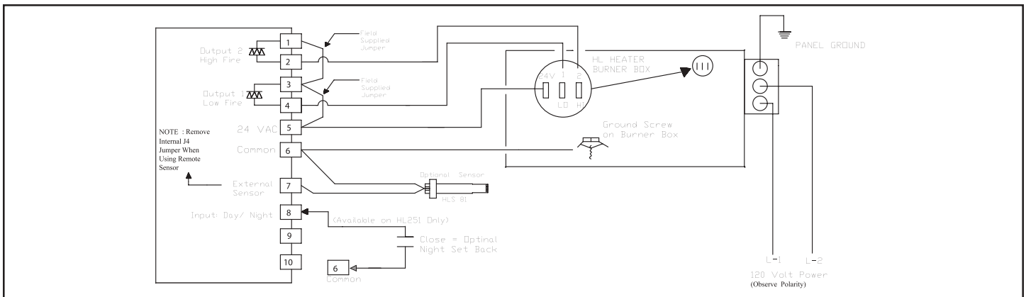
Two-stage heaters with a HL-201 or 251 thermostat. Single heater, single thermostat. No HLRB (relay board) is installed.
