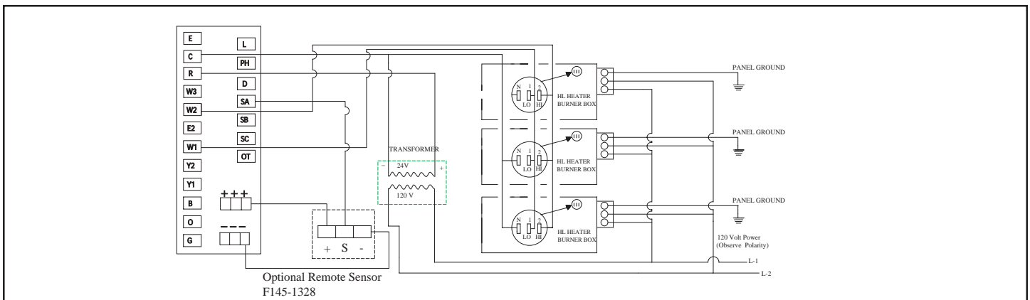
Two-stage heaters with a TH-1F95 thermostat. Single heater, single thermostat. HLRB (relay boards) are installed.
