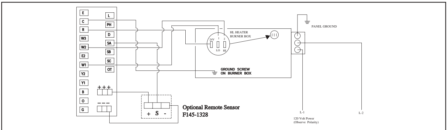
Two-stage heaters with a TH-1F95 thermostat. Single heater, single thermostat. No HLRB (relay board) is installed.
