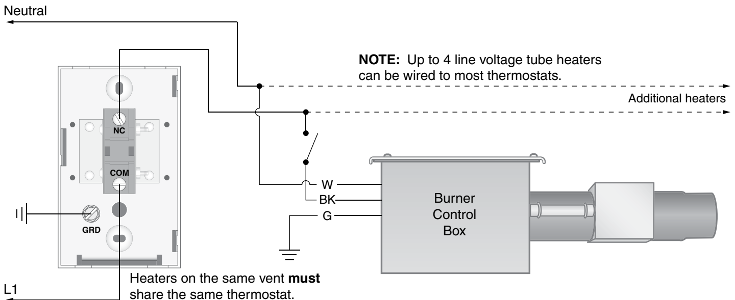
Figure 2 • Typical Field Wiring Diagram - Single line voltage thermostat
