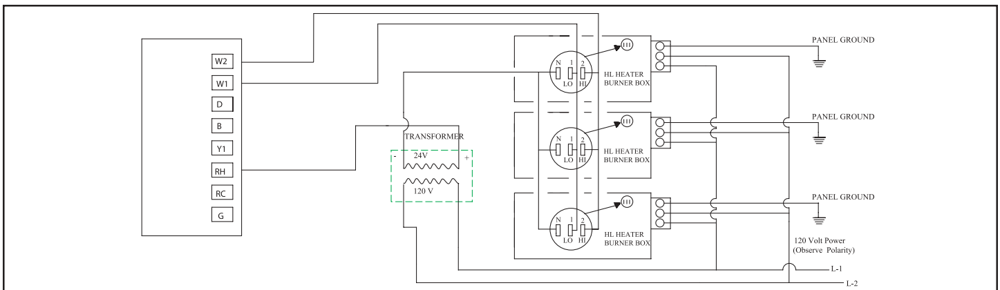
Two-stage heaters with a TH-D152 thermostat. Multiple heaters, single thermostat. HLRB (relay boards) are installed.
