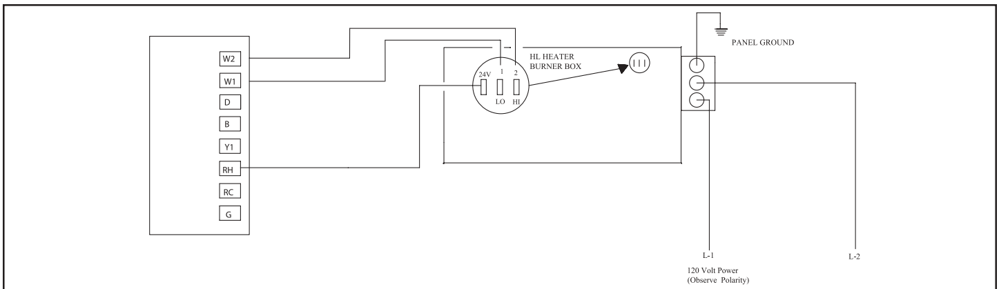
Two-stage heaters with a TH-D152 thermostat. Single heater, single thermostat. No HLRB (relay board) is installed.
