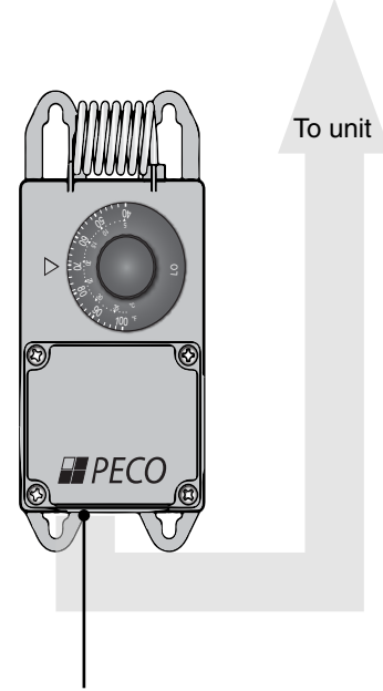
Figure 1 • TH-115 Thermostat
