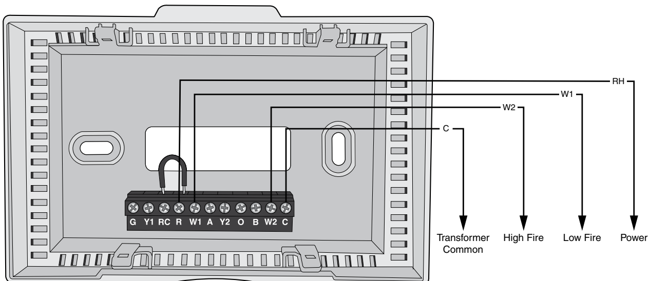
Figure 2 • PSP-722 Thermostat Wiring
