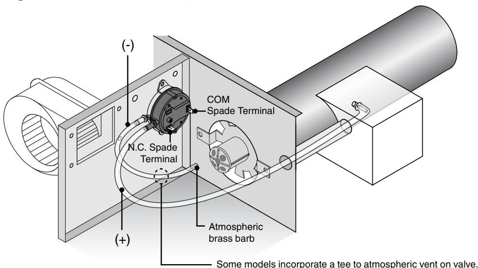
Figure 1 • Exhaust switch replacement for heaters with dual switches
