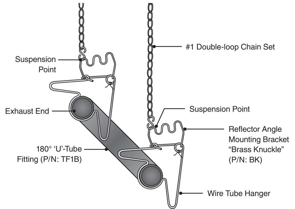
Figure 2 • ‘U’-Tube Angled Hanger Mounting (P/N: TF1B)
