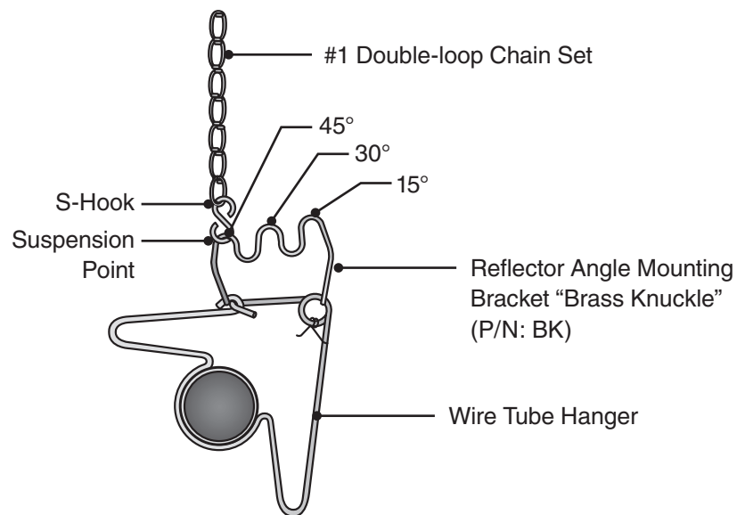
Figure 1 • Straight Tube Angled Hanger Mounting
