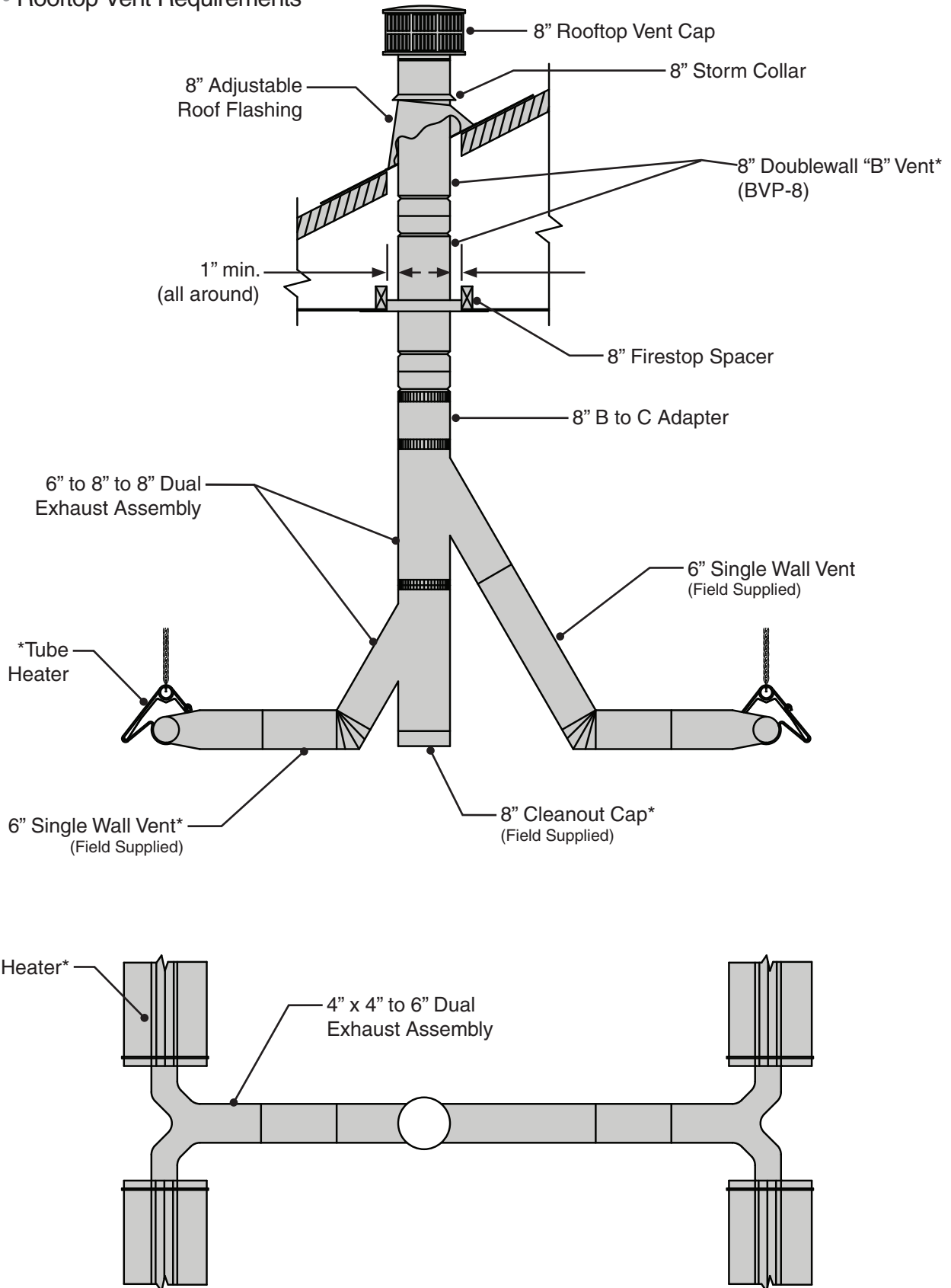
Figure 2 • Rooftop Vent Requirements
