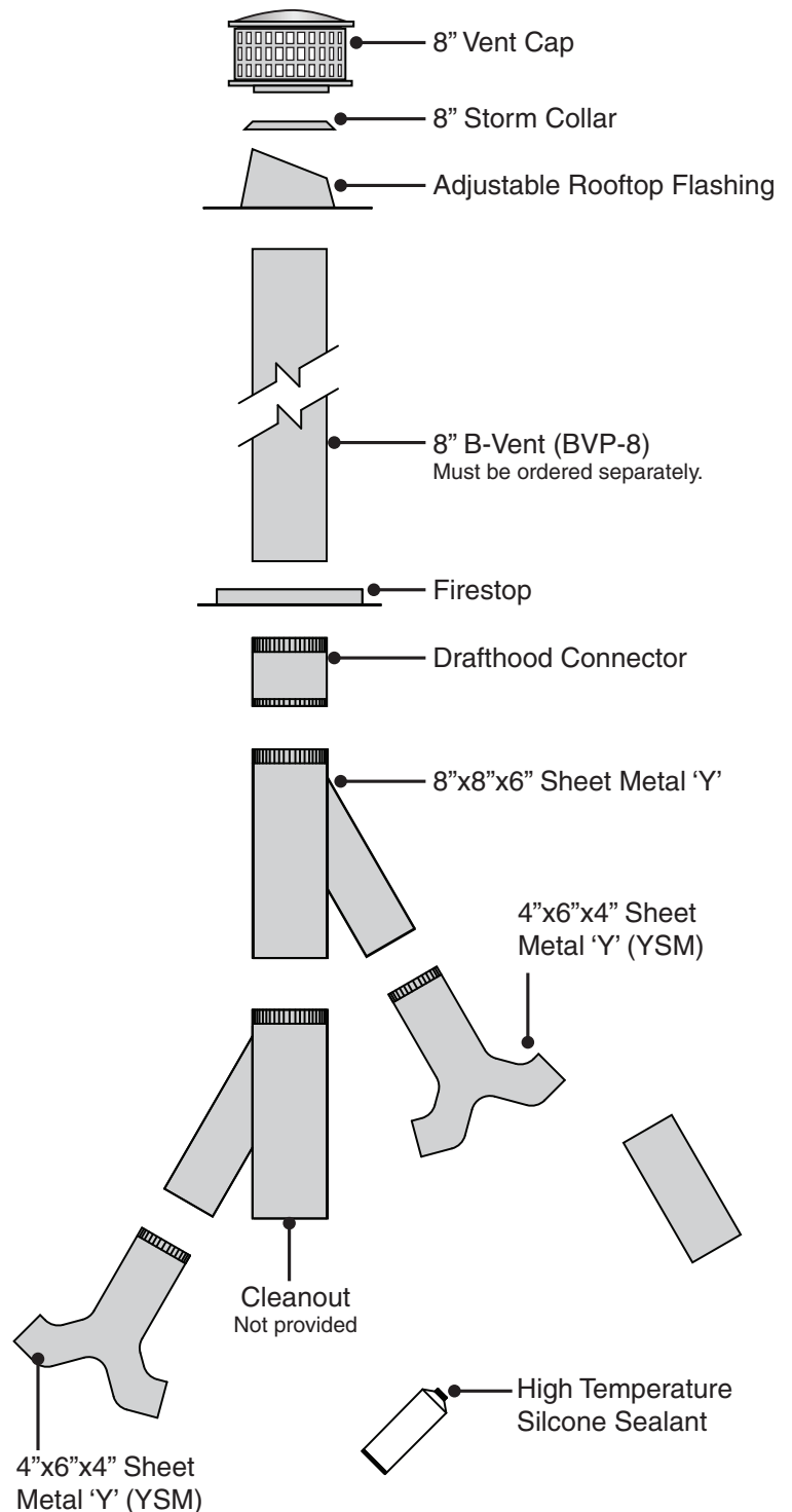
Figure 1 • Kit Contents
