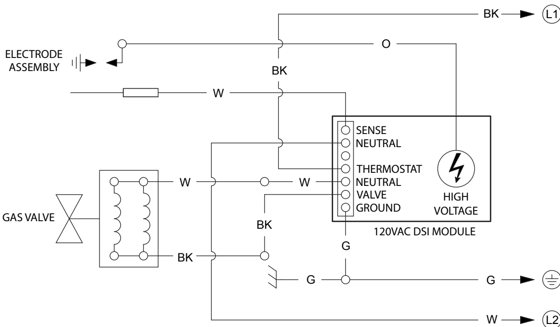
Figure 1 • NFS-2/PFS-2 (120V) Wiring Diagram
