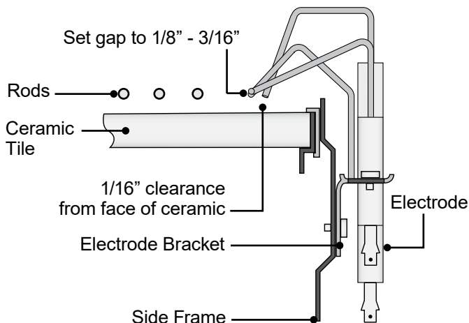
Figure 2 • Replacement 32-508 Electrode Side View
