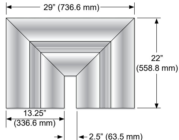
Figure 3 • Reflector 'U' (P/N: RU) Dimensions
