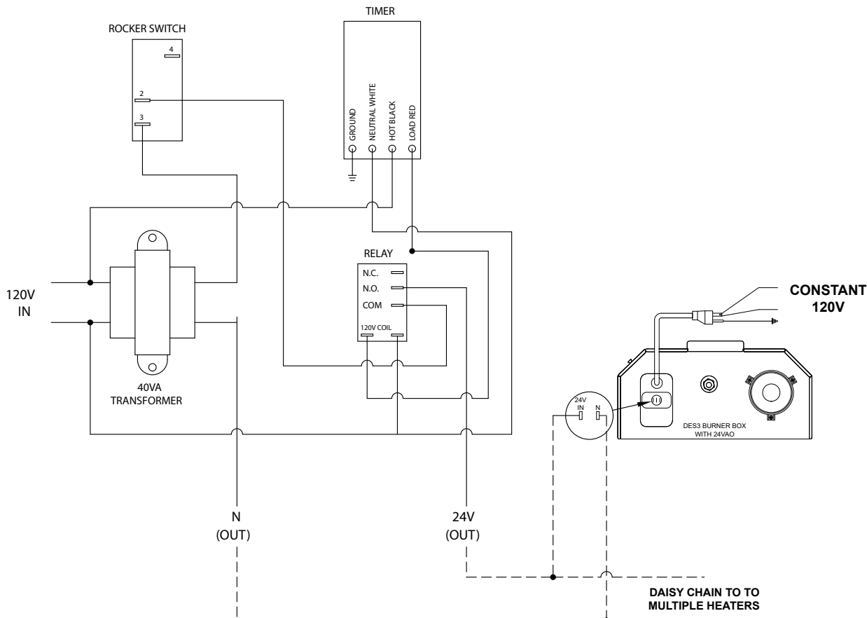
Figure 2 • Single Stage Wiring for Single Heater
