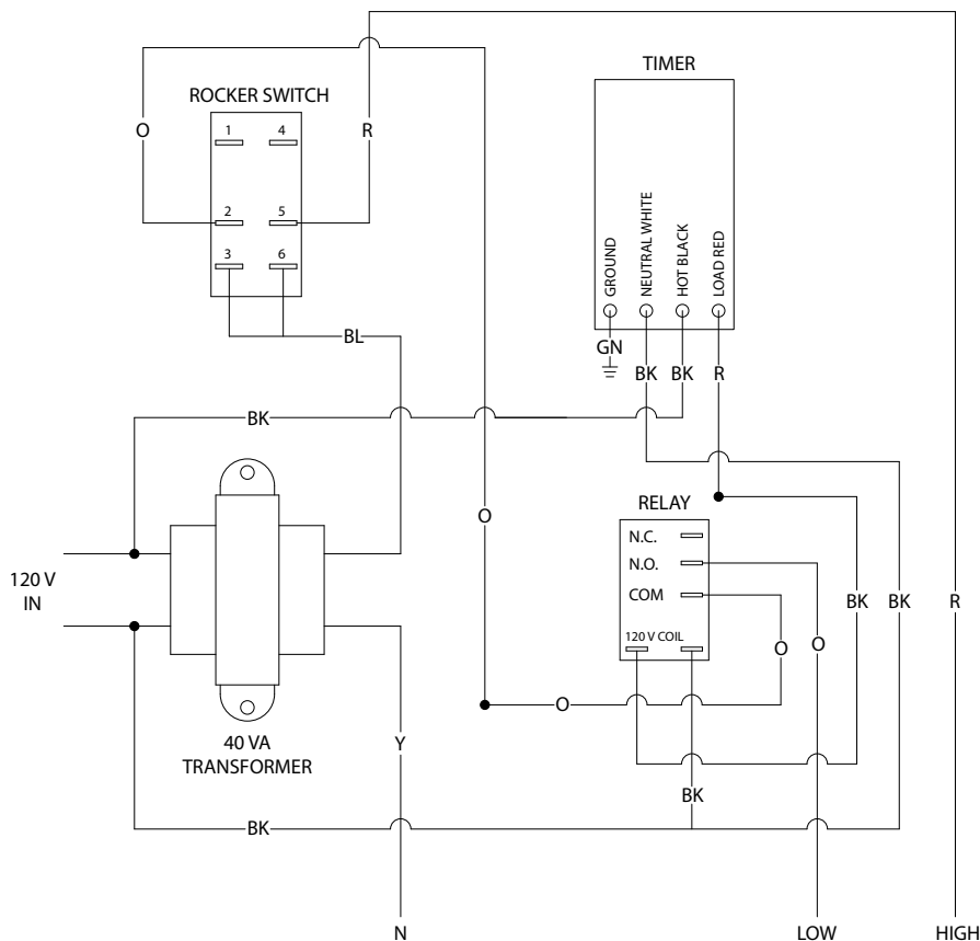
Figure 2 • Two Stage Wiring for Single Heater
