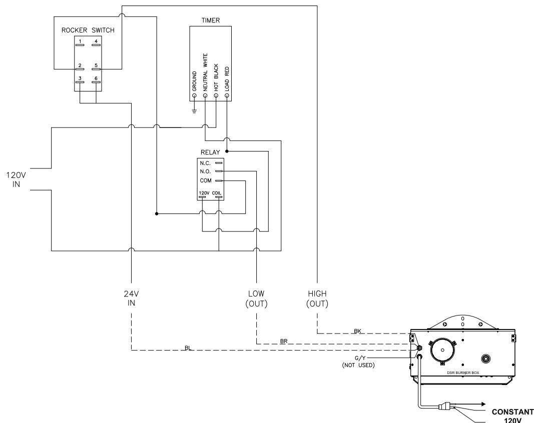
Figure 2 • Two Stage Wiring for Single Heater
