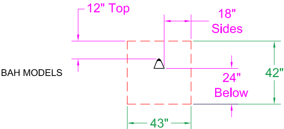
0° Mount - End View
