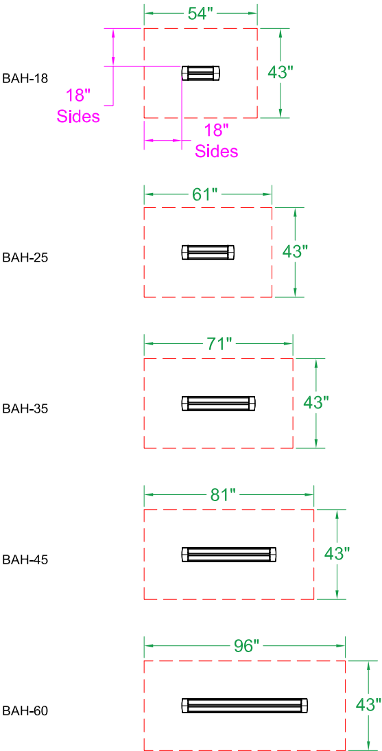
0° Mount - Top View
