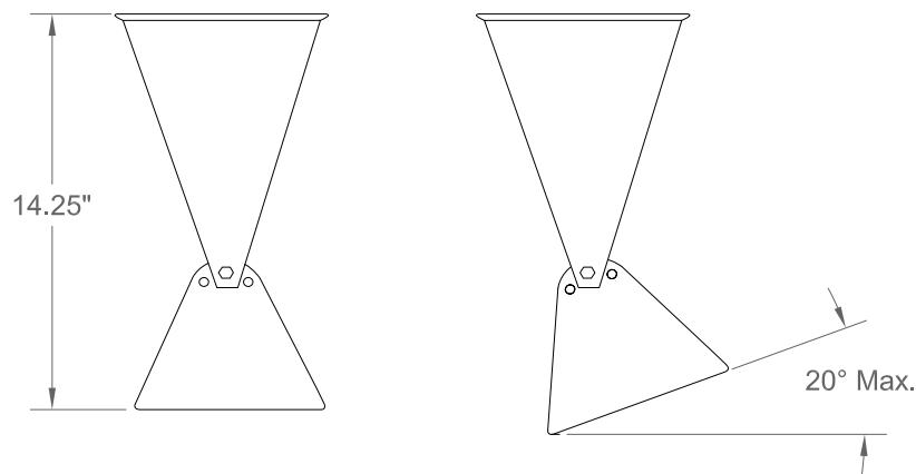
End View with Optional Mounting Bracket
