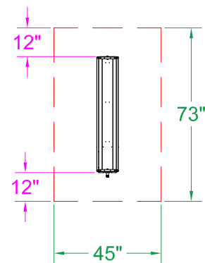
DSC Clearance to Combustible 0° Mount - Top View
