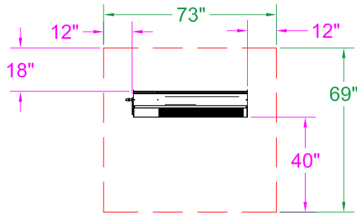
DSC Clearance to Combustible 30° Mount - Front View
