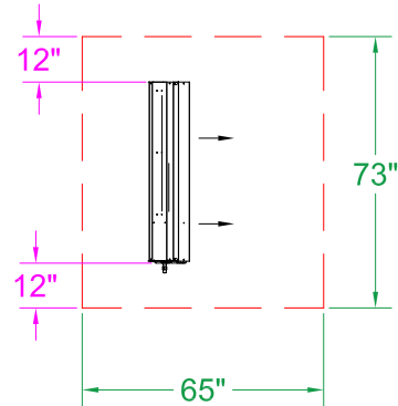
DSC Clearance to Combustible 30° Mount - Top View
