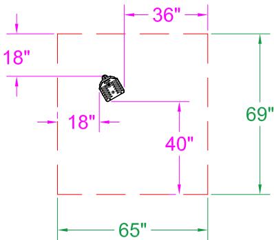
DSC Clearance to Combustible 30° Mount - End View
