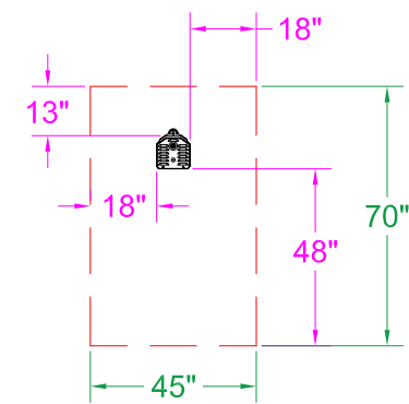
DSC Clearance to Combustible 0° Mount - End View
