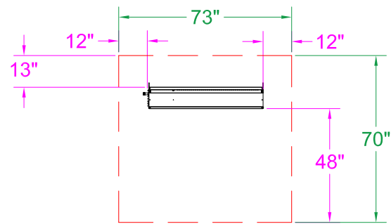
DSC Clearance to Combustible 0° Mount - Front View
