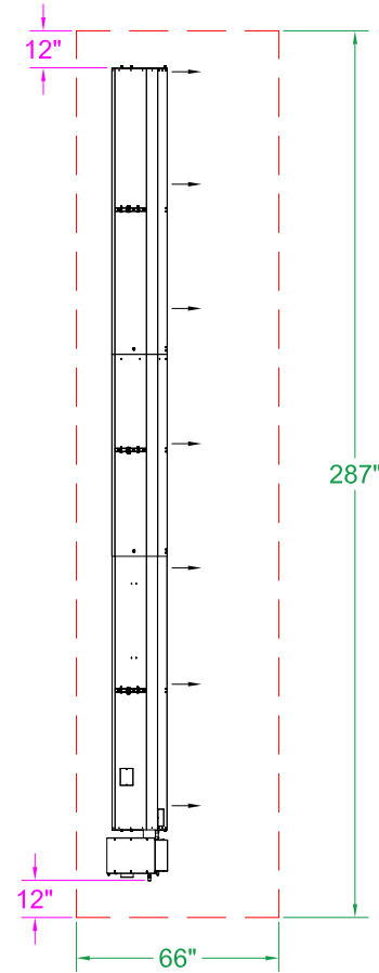
DSRF-35-65 & 80 Clearance to Combustible 30° Mount - Top View
