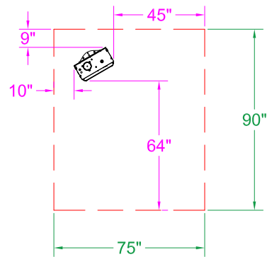
DSRF-35-100 Clearance to Combustible 30° Mount - End View
