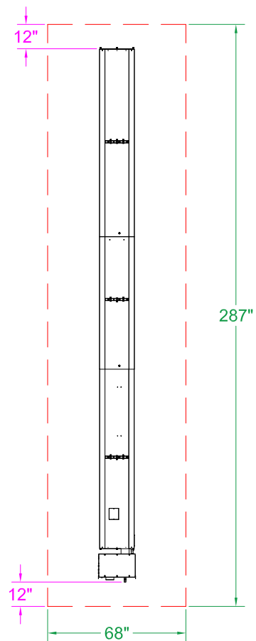
DSRF-35-65 & 80 Clearance to Combustible 0° Mount - Top View
