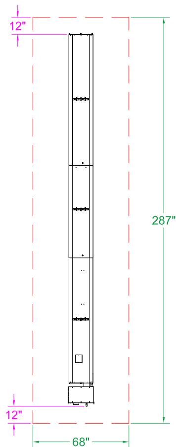
DSRF-35-100 Clearance to Combustible 0° Mount - Top View
