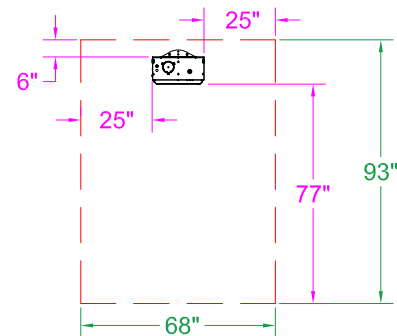
DSRF-35-100 Clearance to Combustible 0° Mount - End View
