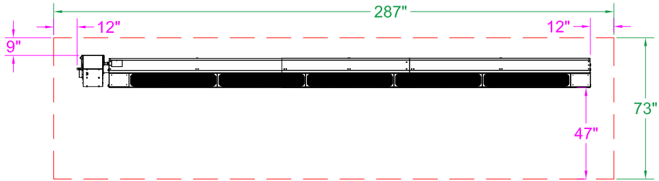
DSRF-35-65 & 80 Clearance to Combustible 30° Mount - Front View
