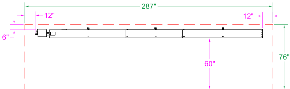
DSRF-35-65 & 80 Clearance to Combustible 0° Mount - Front View
