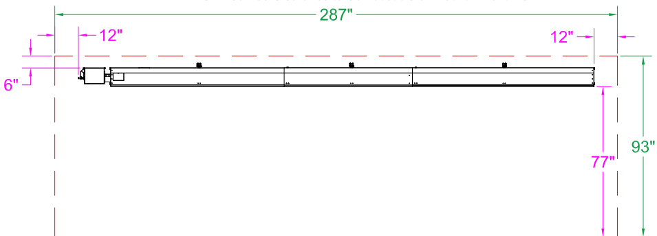
DSRF-35-100 Clearance to Combustible 0° Mount - Front View
