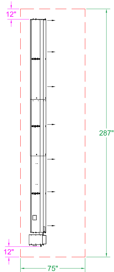
DSRF-35-100 Clearance to Combustible 30° Mount - Top View
