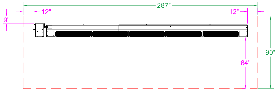
DSRF-35-100 Clearance to Combustible 30° Mount - Front View
