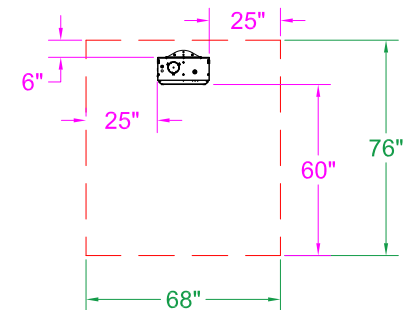
DSRF-35-65 & 80 Clearance to Combustible 0° Mount - Top View
