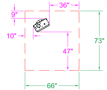
DSRF-35-65 & 80 Clearance to Combustible 30° Mount - Top View
