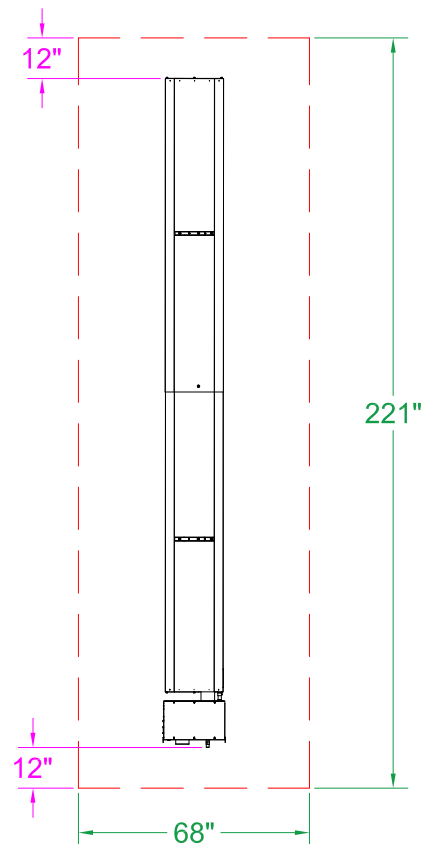
DSRL-100 Clearance to Combustible 0° Mount - Top View
