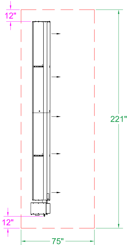
DSRL-100 Clearance to Combustible 30° Mount - Top View
