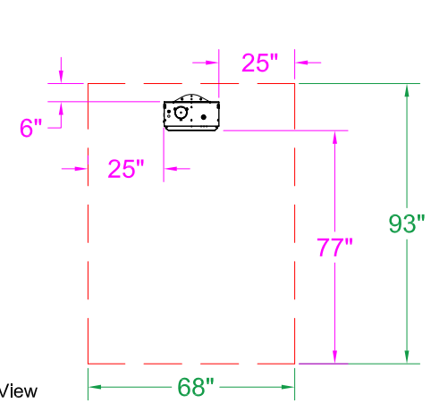
DSRL-100 Clearance to Combustible 0° Mount - End View
