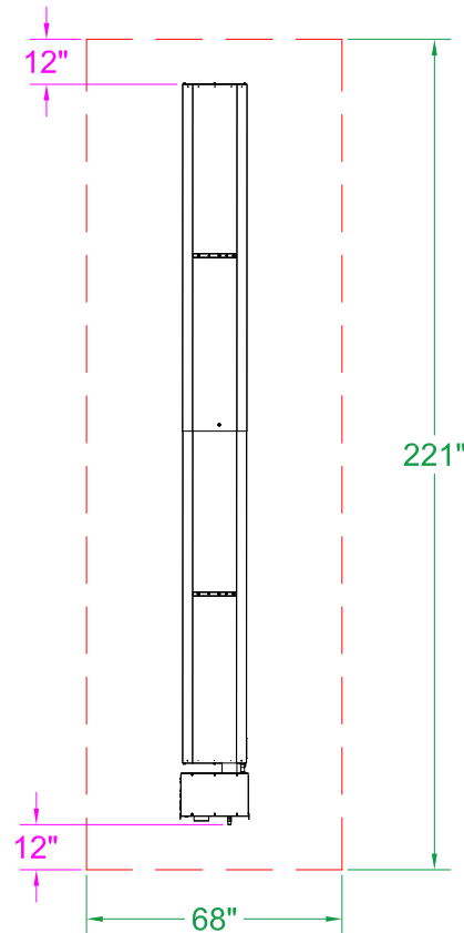
DSRL-65 & 80 Clearance to Combustible 0° Mount - Top View
