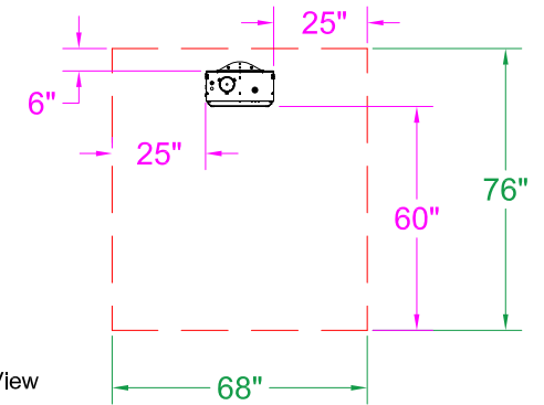
DSRL-65 & 80 Clearance to Combustible 0° Mount - End View
