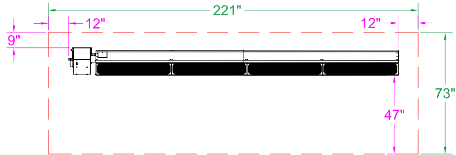
DSRL-65 & 80 Clearance to Combustible 30° Mount - Front View
