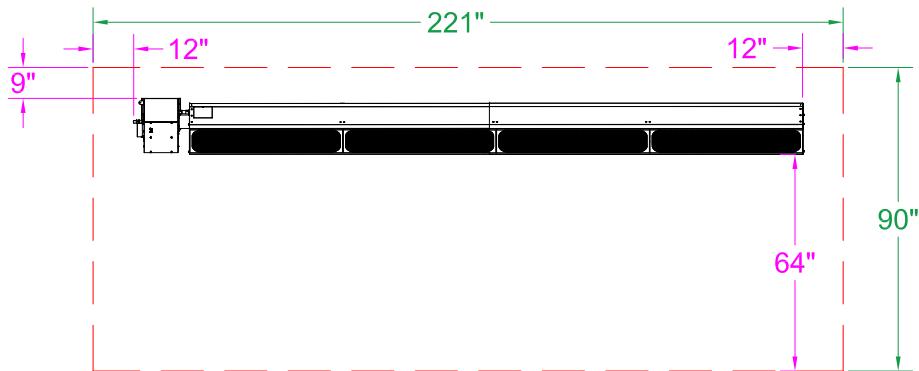
DSRL-100 Clearance to Combustible 30° Mount - Front View
