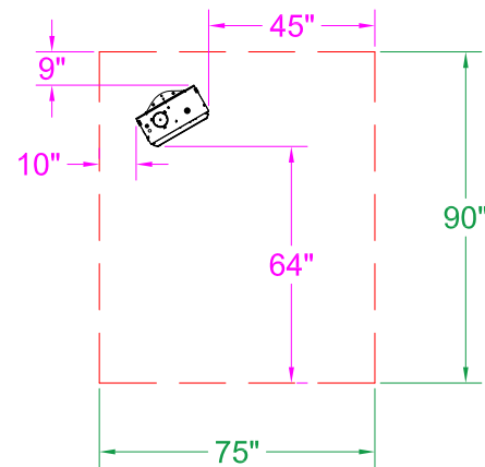
DSRL-100 Clearance to Combustible 30° Mount - End View
