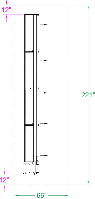
DSRL-65 & 80 Clearance to Combustible 30° Mount - Top View
