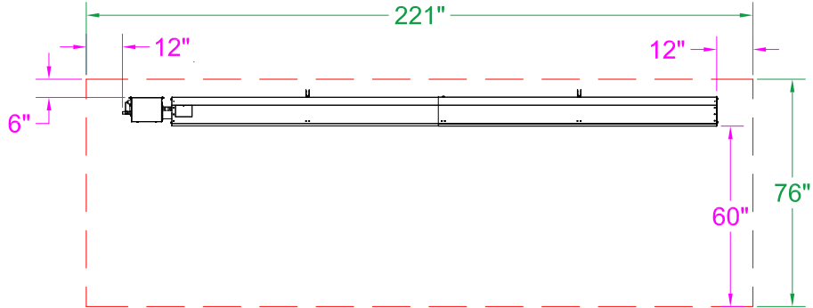
DSRL-65 & 80 Clearance to Combustible 0° Mount - Front View
