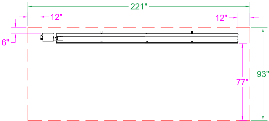
DSRL-100 Clearance to Combustible 0° Mount - Front View
