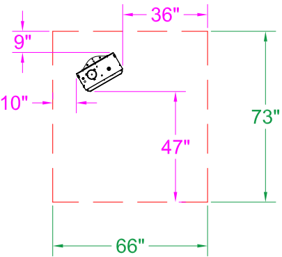
DSRL-65 & 80 Clearance to Combustible 30° Mount - Top View
