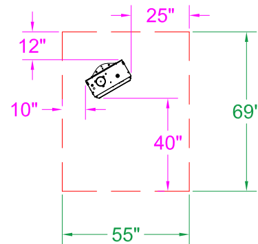
DSRS-50 Clearance to Combustible 30° Mount - End View
