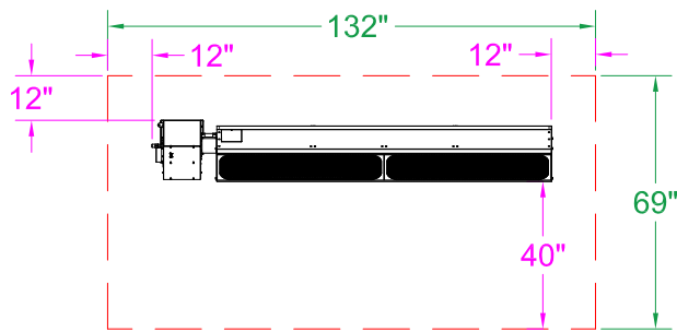
DSRS-50 Clearance to Combustible 30° Mount - Front View
