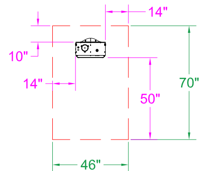
DSRS-50 Clearance to Combustible 0° Mount - End View
