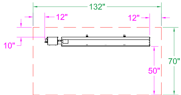
DSRS-50 Clearance to Combustible 0° Mount - Front View
