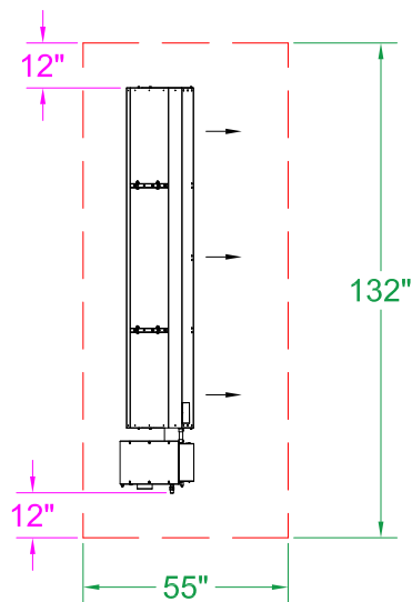
DSRS-50 Clearance to Combustible 30° Mount - Top View
