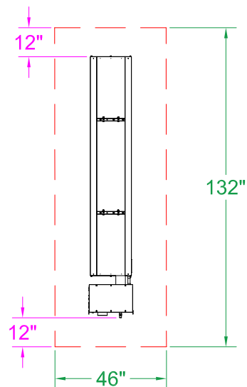
DSRS-50 Clearance to Combustible 0° Mount - Top View
