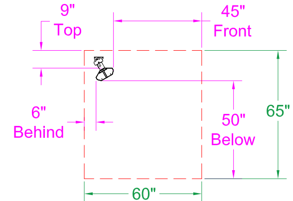
30° Mount - End View
