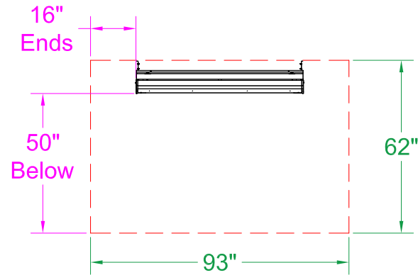
0° Mount - Side View
