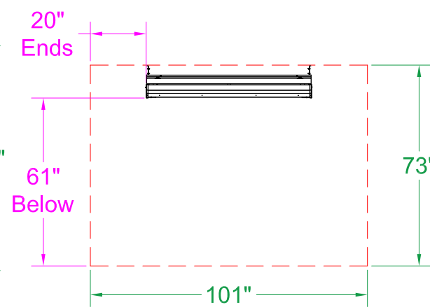
30° Mount - Front View
