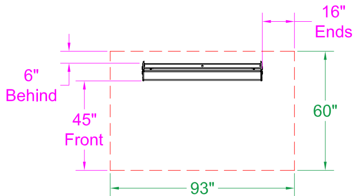
30° Mount - Top View
