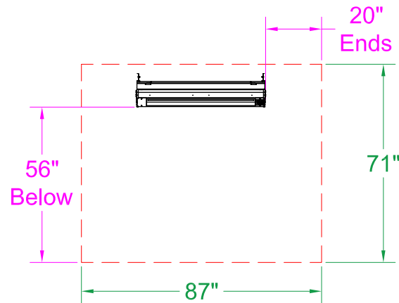
30° Mount - Front View
