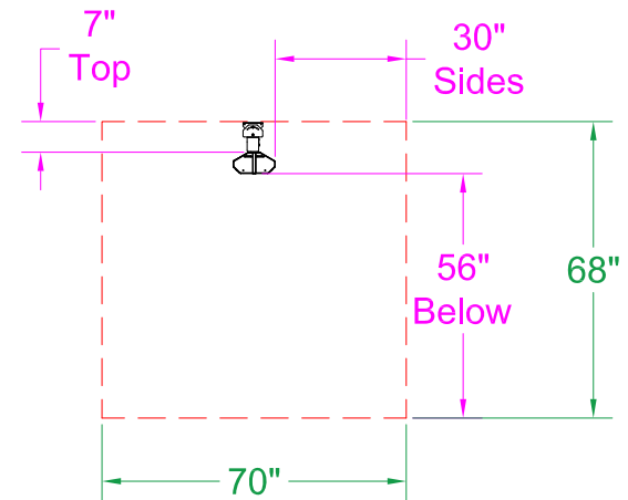
0° Mount - End View
