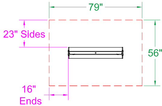
0° Mount - Top View
