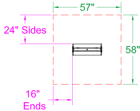
30° Mount - Top View
