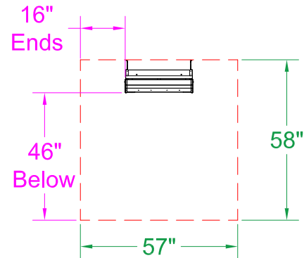
0° Mount - Side View
