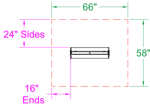
0° Mount - Top View
