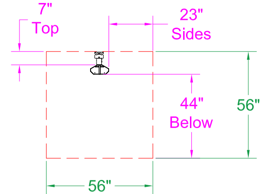
0° Mount - End View
