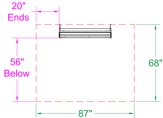
30° Mount - Front View
