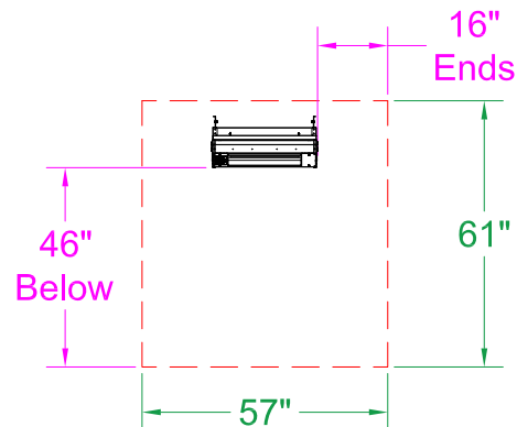
30° Mount - Front View
