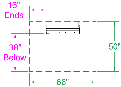
0° Mount - Side View
