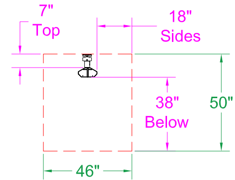
0° Mount - End View
