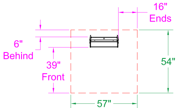
30° Mount - Top View
