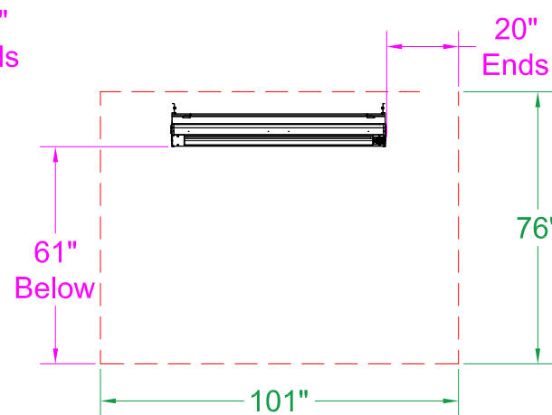
30° Mount - Front View
