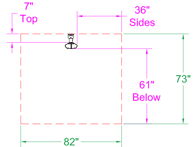
30° Mount - End View
