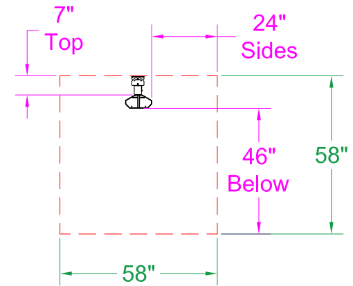
0° Mount - End View
