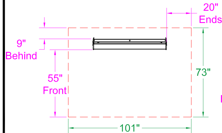
30° Mount - Top View
