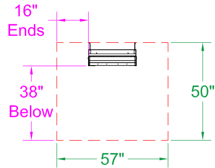
0° Mount - Side View
