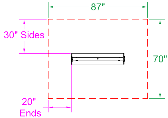
30° Mount - Top View
