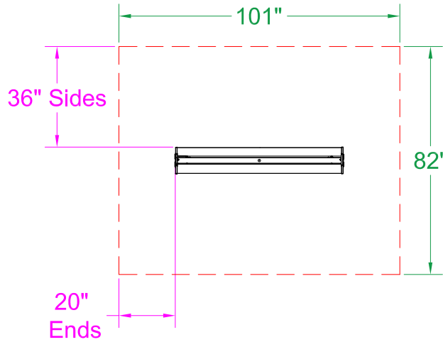
30° Mount - Top View
