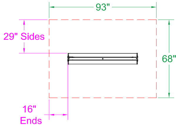
30° Mount - Top View
