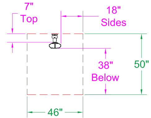
0° Mount - End View
