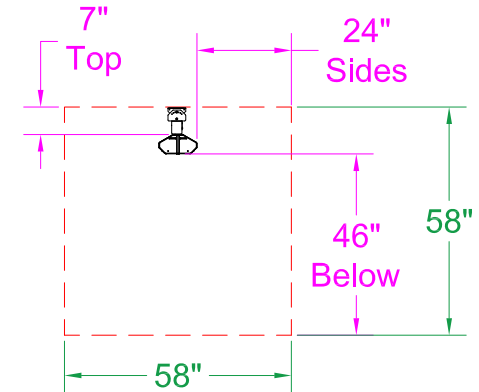
0° Mount - End View
