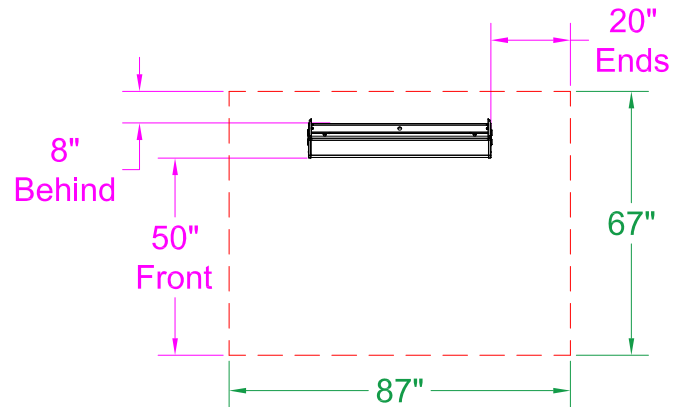
30° Mount - Top View
