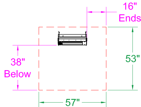
30° Mount - Front View
