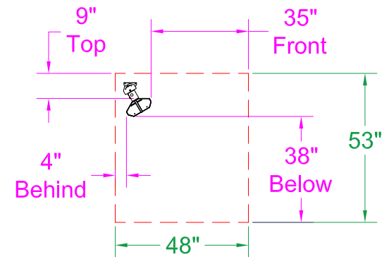
30° Mount - End View
