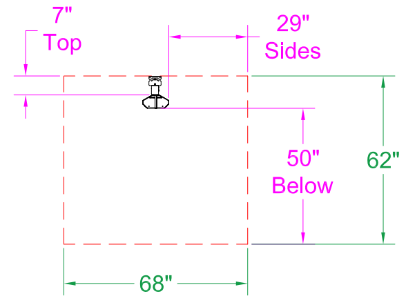
0° Mount - End View
