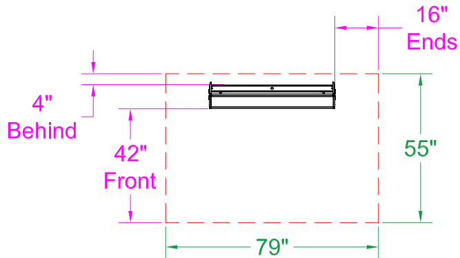
30° Mount - Top View
