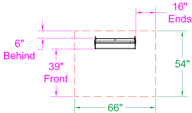
30° Mount - Top View
