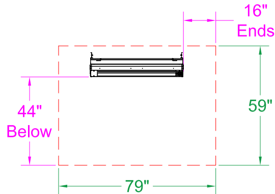
30° Mount - Front View
