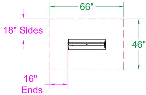
0° Mount - Top View
