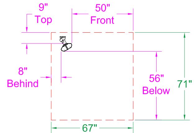
30° Mount - End View
