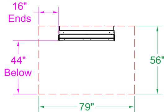
0° Mount - Side View
