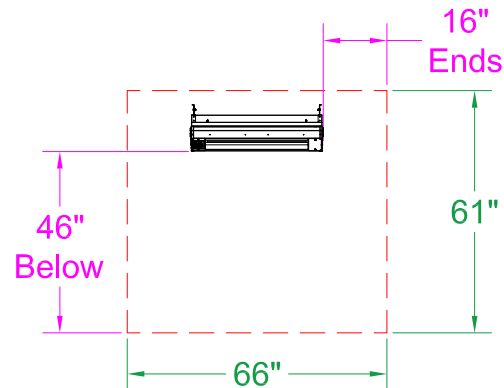
30° Mount - Front View
