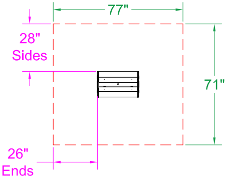
0° Mount - Top View
