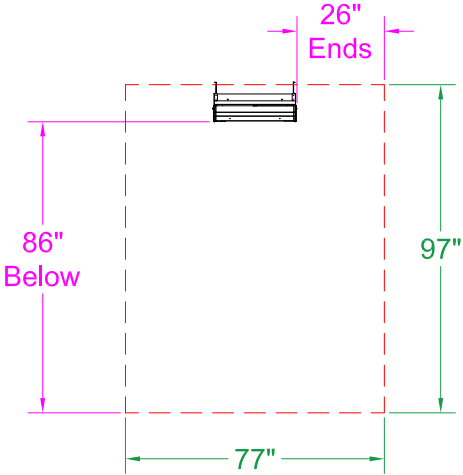
0° Mount - Side View
