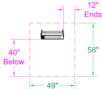
45° Mount - Front View
