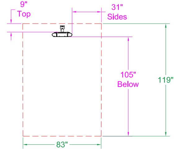
0° Mount - End View
