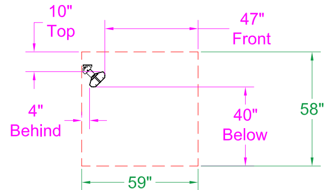
45° Mount - End View
