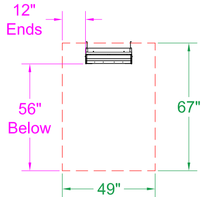
0° Mount - Side View
