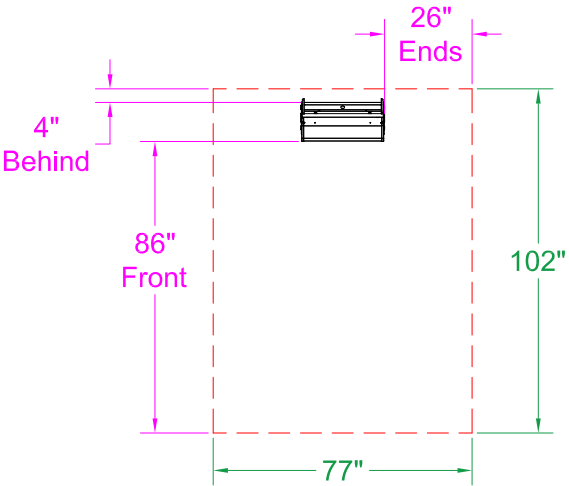
45° Mount - Top View
