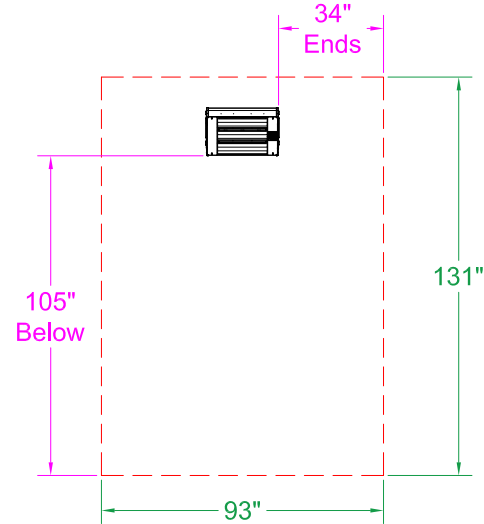
45° Mount - Front View
