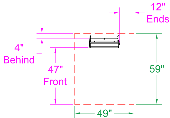
45° Mount - Top View
