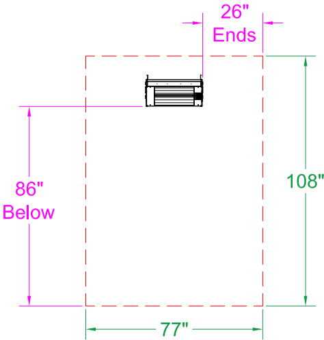
45° Mount - Front View
