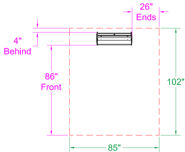
45° Mount - Top View
