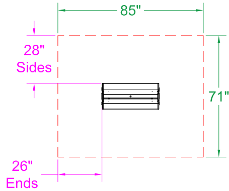
0° Mount - Top View
