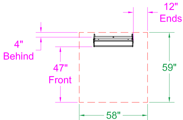
45° Mount - Top View
