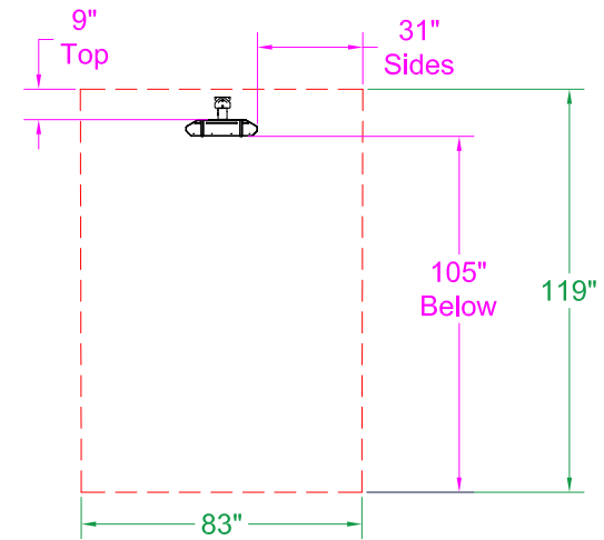
0° Mount - End View
