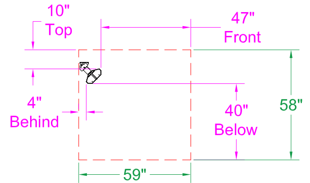
45° Mount - End View
