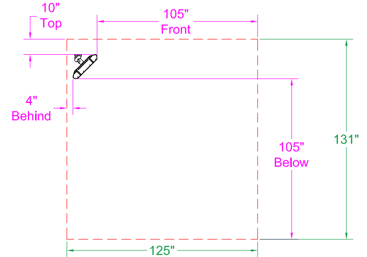
45° Mount - End View
