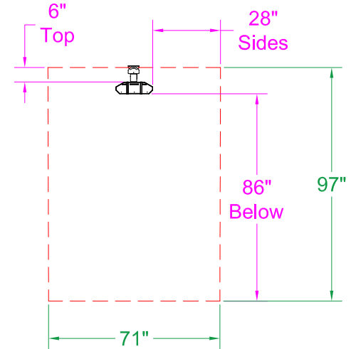
0° Mount - End View
