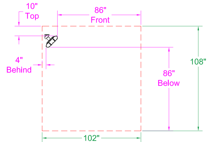
45° Mount - End View
