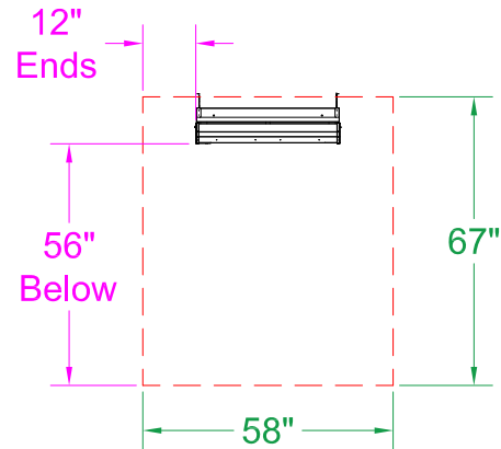
0° Mount - Side View
