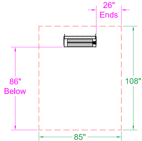
45° Mount - Front View
