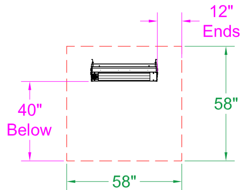
45° Mount - Front View
