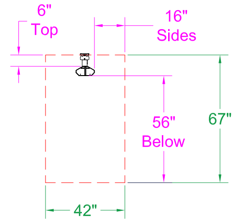
0° Mount - End View
