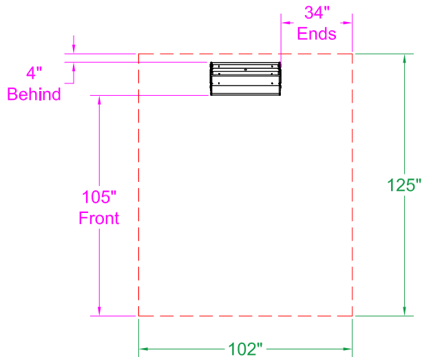
45° Mount - Top View
