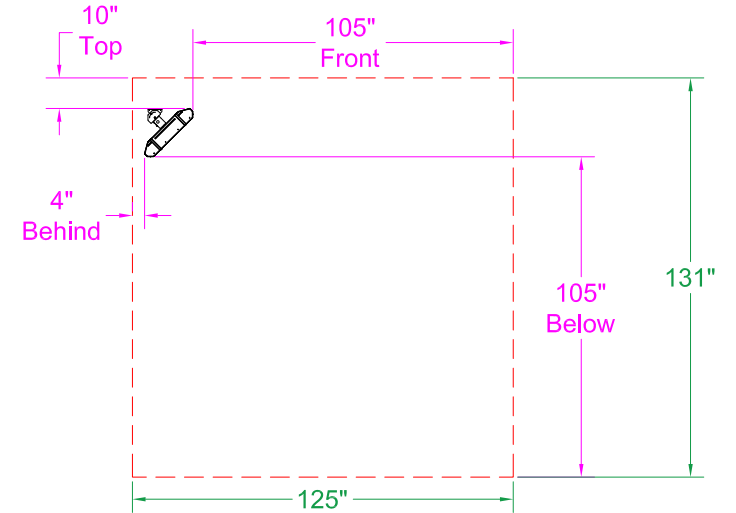
45° Mount - End View
