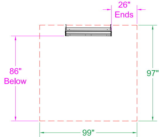
0° Mount - Side View
