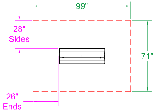
0° Mount - Top View
