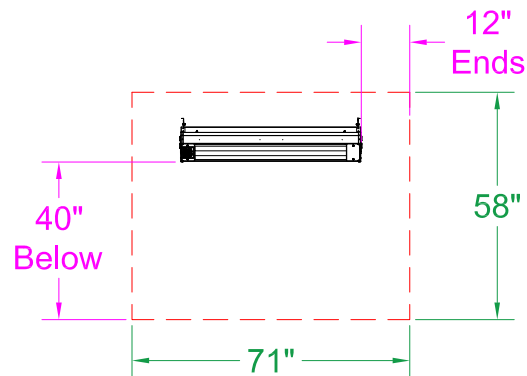
45° Mount - Front View
