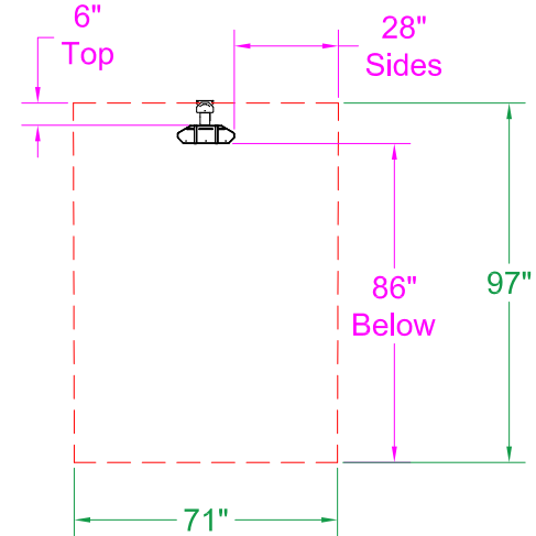
0° Mount - End View
