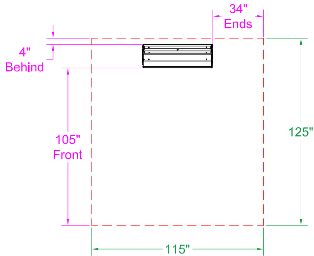
45° Mount - Top View
