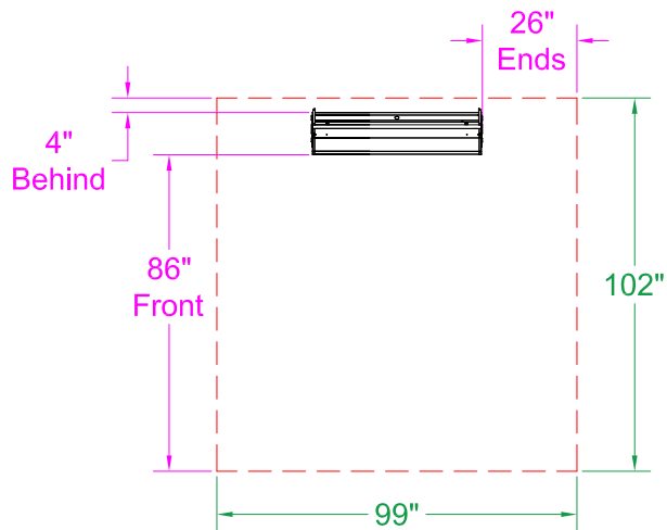
45° Mount - Top View
