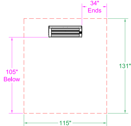
45° Mount - Front View
