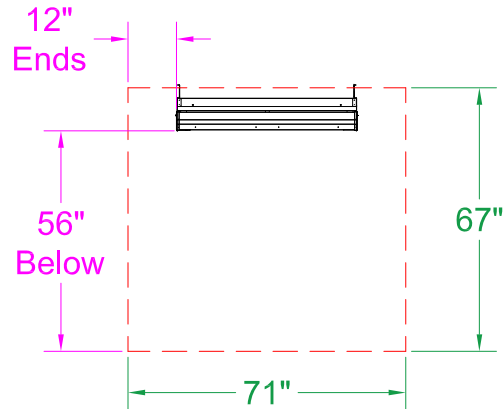
0° Mount - Side View
