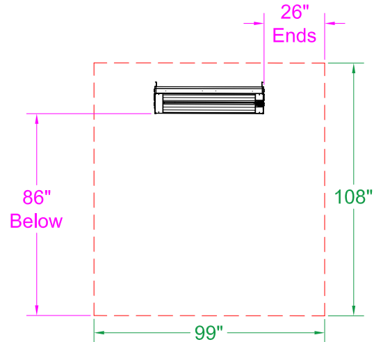
45° Mount - Front View
