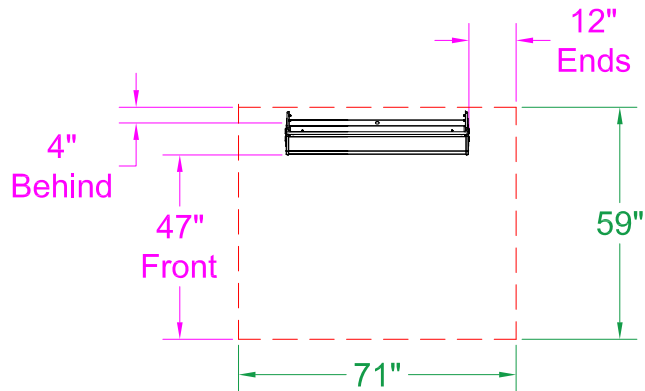
45° Mount - Top View
