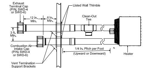
Outside Combustion Air Sidewall Intake
