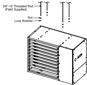
FA-100 to FA-250 Mounting
