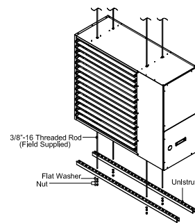
FA-300 and FA-400 Mounting
