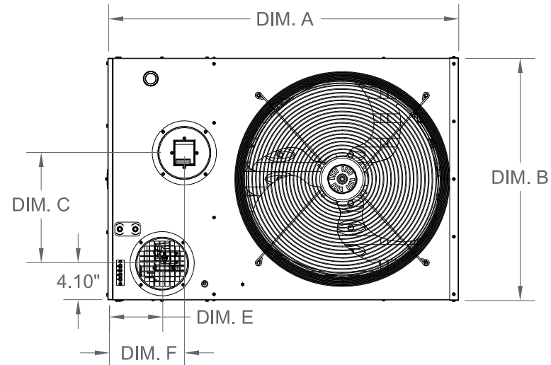
Rear View
