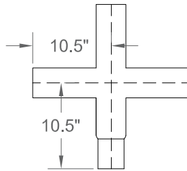
Cross (P/N: V-CR)
